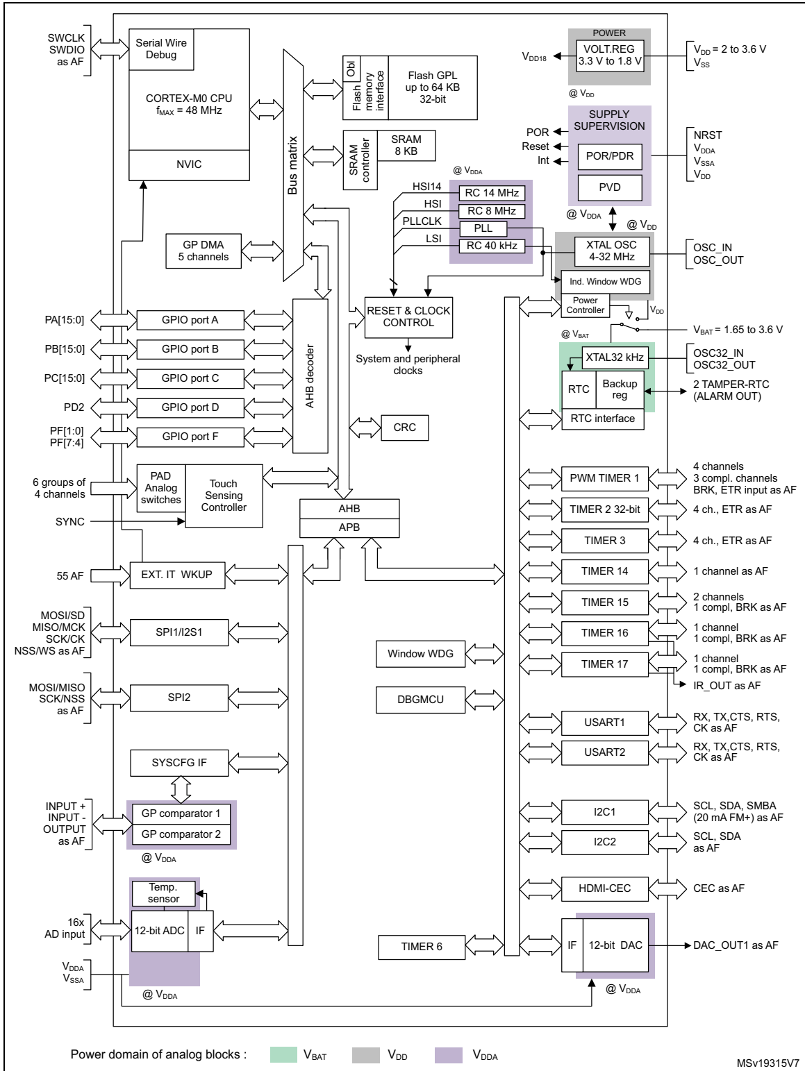
Figure 1. Block diagram
