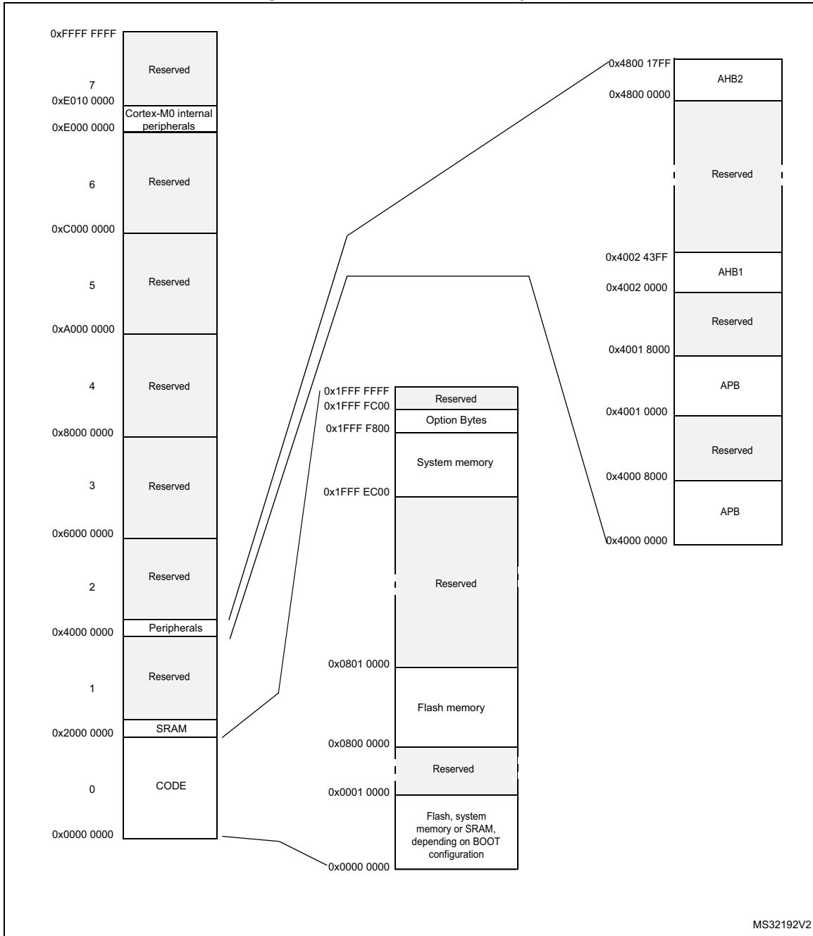
Figure 10. STM32F051x8 memory map
