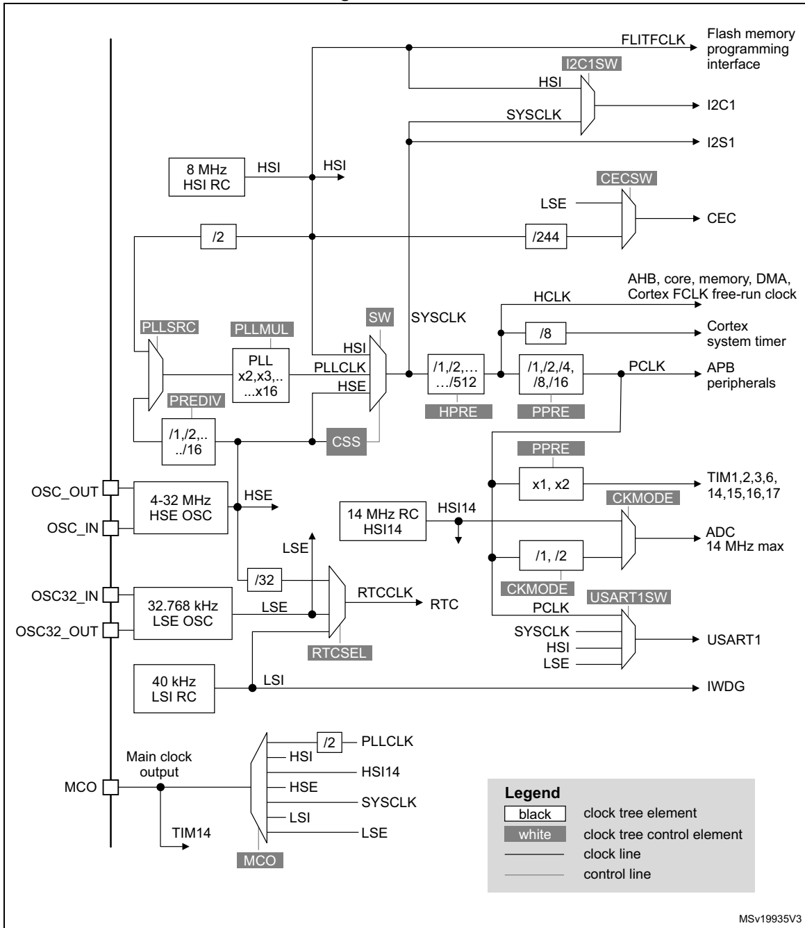
Figure 2. Clock tree
